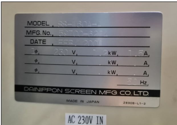
type plate SS-W60A-A
